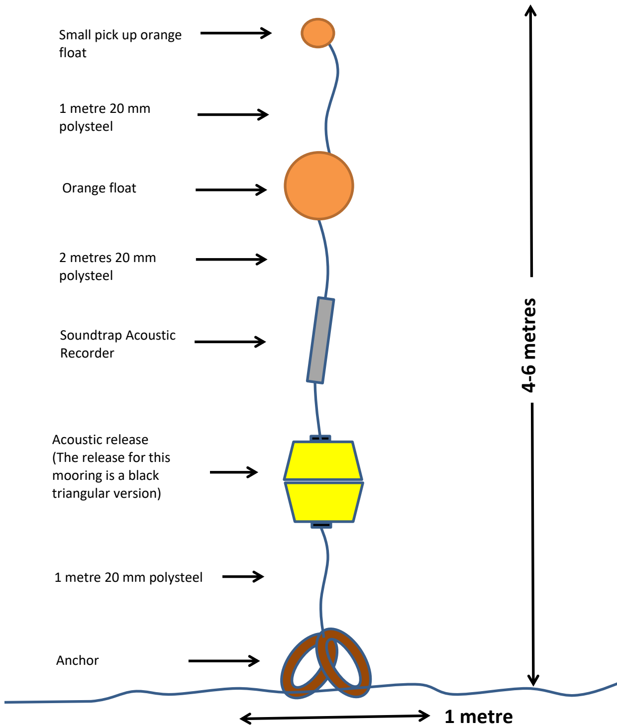
Drawing presenting passive acoustic monitoring mooring design
